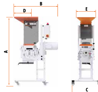
Sprue picker hopper
